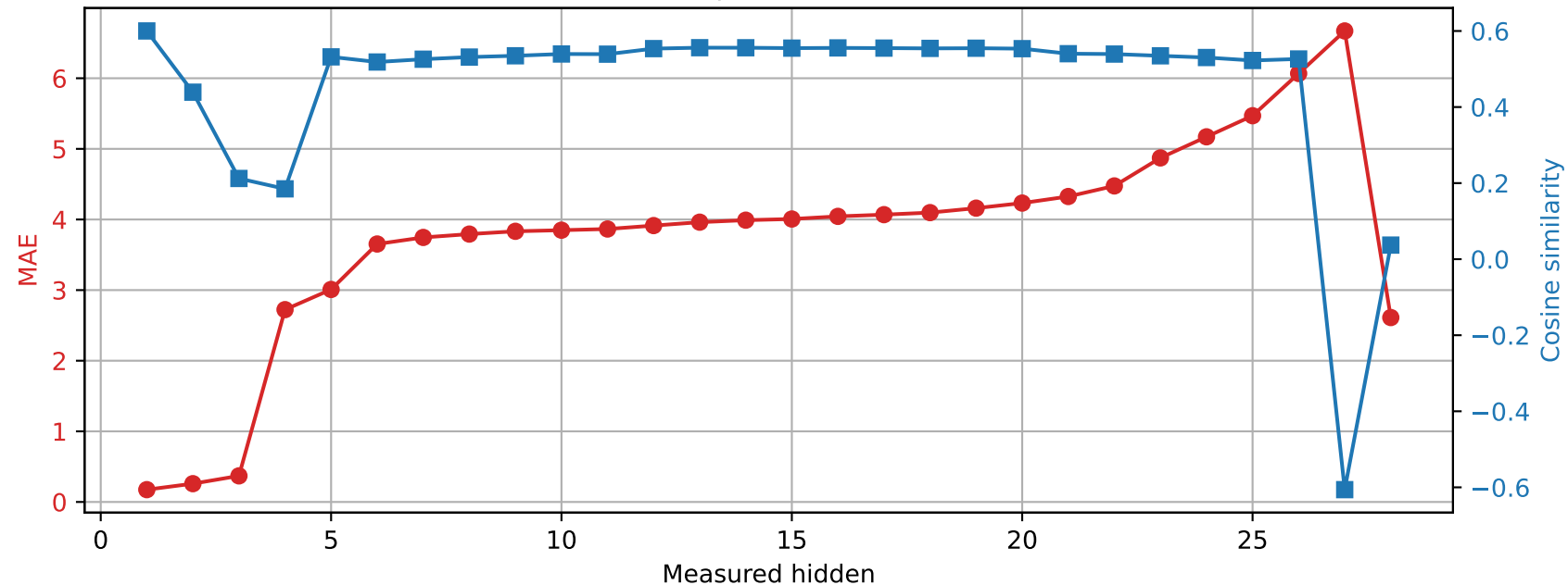
Qwen2.5-7B-Instruct | Prompt 3 Spared layer 22 | Unquantized vs hybrid
