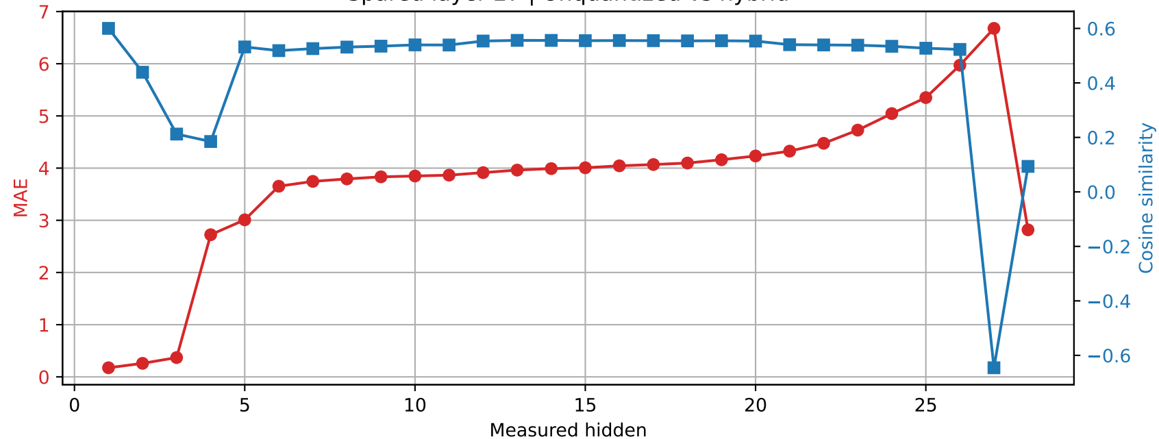
Qwen2.5-7B-Instruct | Prompt 3 Spared layer 27 | Unquantized vs hybrid
