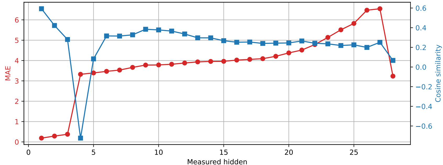
Qwen2.5-7B-Instruct | Prompt 4 Spared layer 3 | Unquantized vs hybrid
