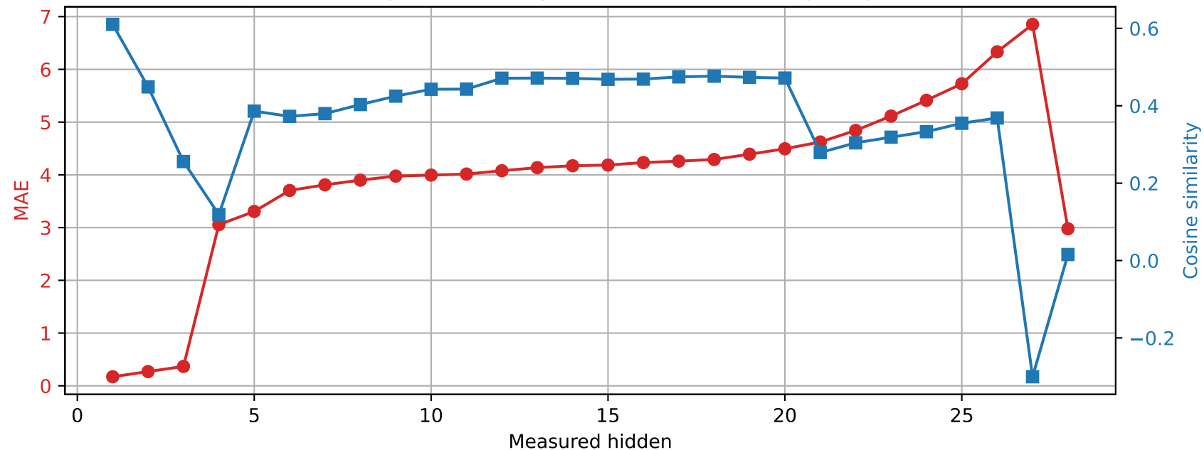
Qwen2.5-7B-Instruct Mean unquantized vs quantized int4 across 5 prompts
