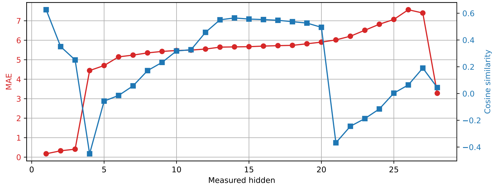
Qwen2.5-7B-Instruct | Prompt 0 Spared layer 12 | Unquantized vs hybrid
