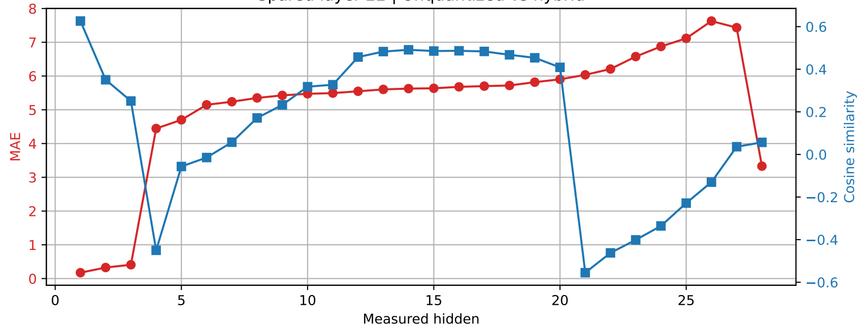
Qwen2.5-7B-Instruct | Prompt 0 Spared layer 22 | Unquantized vs hybrid
