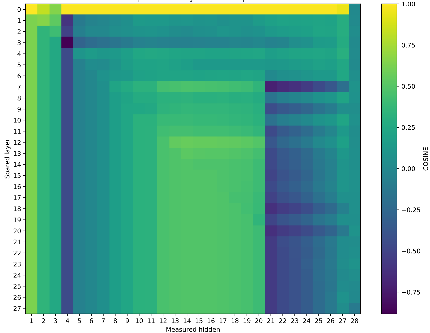
Qwen2.5-7B-Instruct | Prompt 0 Unquantized vs hybrid cos sim | int4
