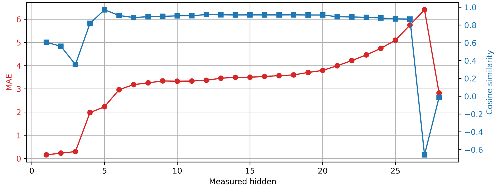
Qwen2.5-7B-Instruct | Prompt 1 Spared layer 12 | Unquantized vs hybrid
