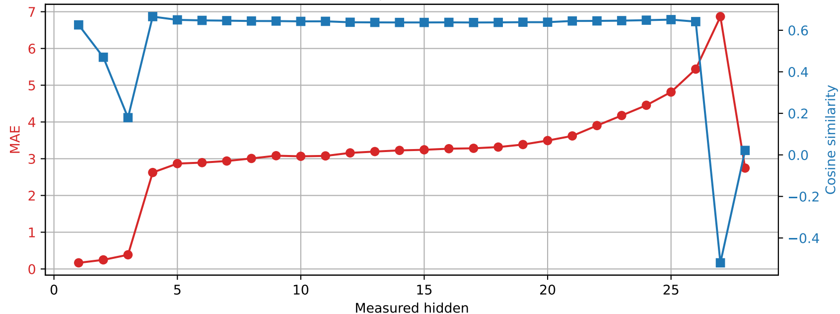
Qwen2.5-7B-Instruct | Prompt 2 Spared layer 3 | Unquantized vs hybrid
