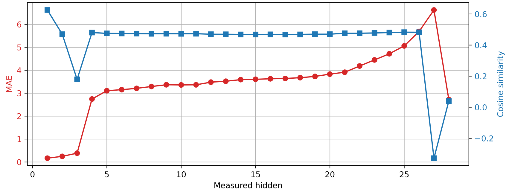
Qwen2.5-7B-Instruct | Prompt 2 Spared layer 13 | Unquantized vs hybrid
