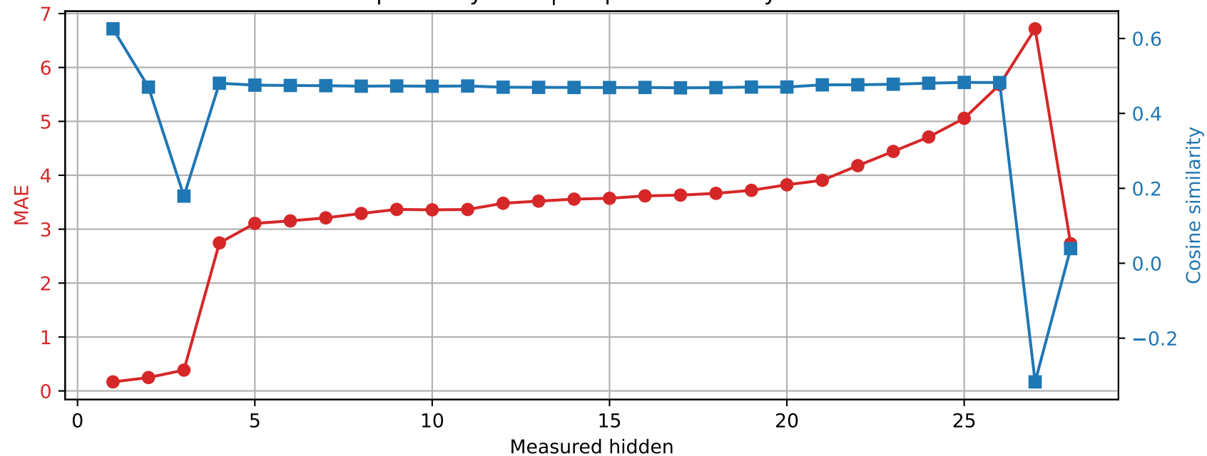
Qwen2.5-7B-Instruct | Prompt 2 Spared layer 15 | Unquantized vs hybrid
