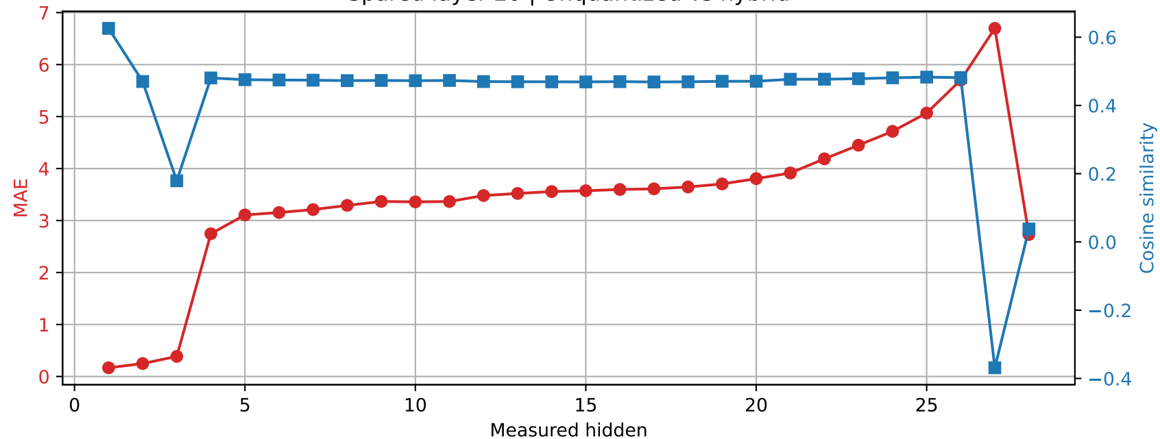
Qwen2.5-7B-Instruct | Prompt 2 Spared layer 20 | Unquantized vs hybrid
