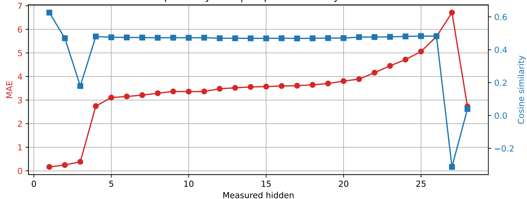
Qwen2.5-7B-Instruct | Prompt 2 Spared layer 22 | Unquantized vs hybrid
