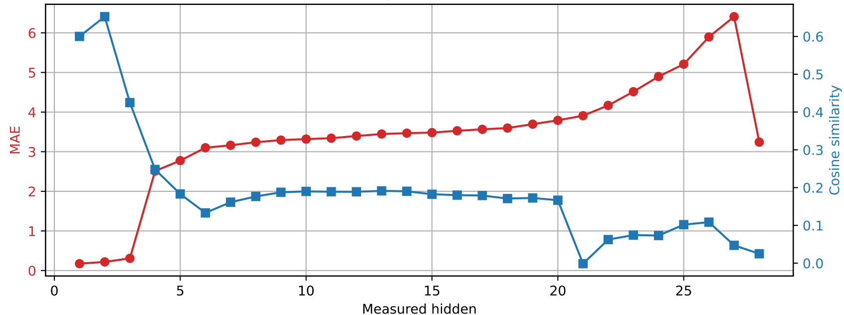
Qwen2.5-7B-Instruct | Prompt 3 Spared layer 1 | Unquantized vs hybrid
