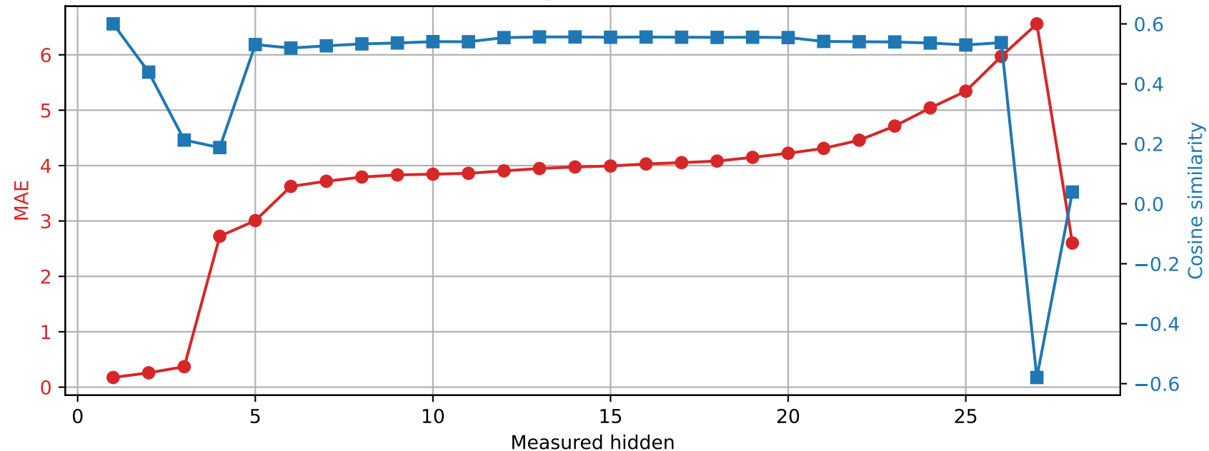
Qwen2.5-7B-Instruct | Prompt 3 Spared layer 7 | Unquantized vs hybrid
