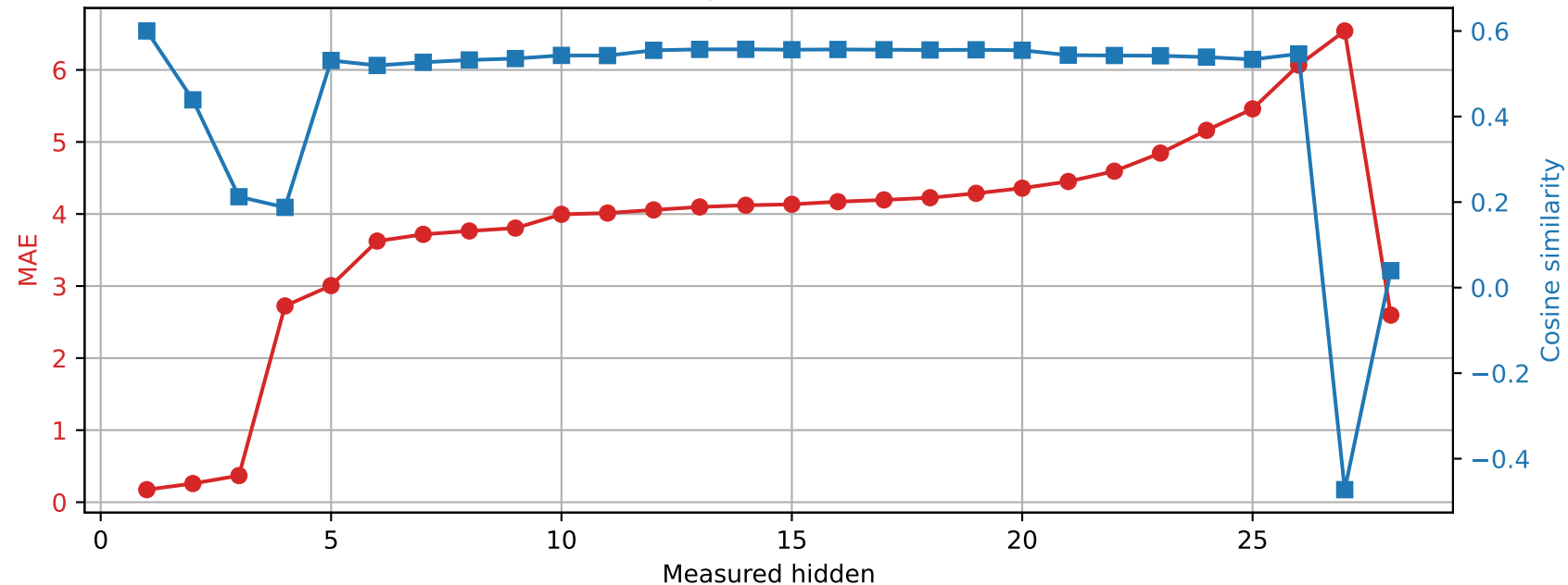
Qwen2.5-7B-Instruct | Prompt 3 Spared layer 9 | Unquantized vs hybrid
