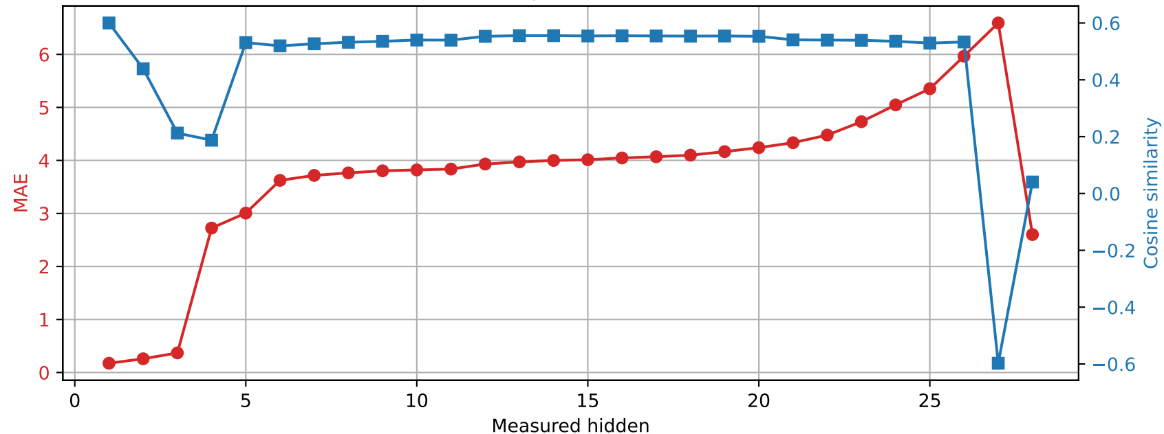
Qwen2.5-7B-Instruct | Prompt 3 Spared layer 11 | Unquantized vs hybrid
