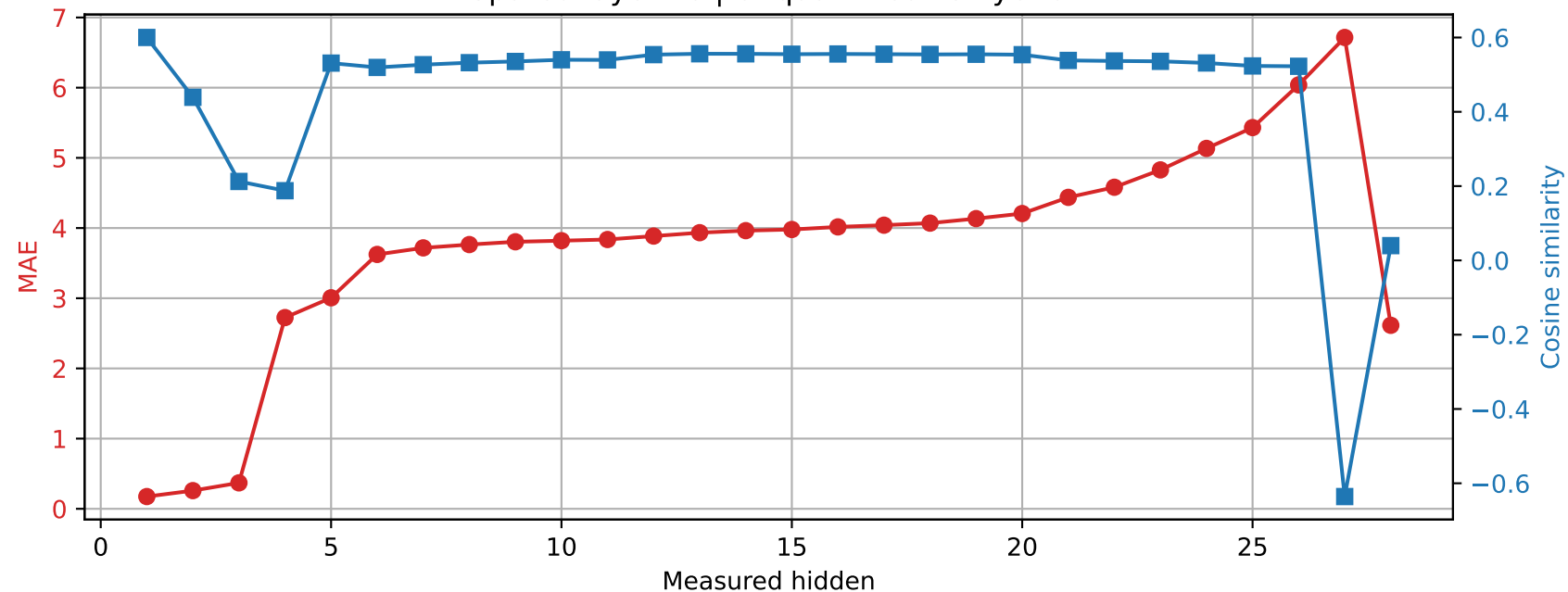
Qwen2.5-7B-Instruct | Prompt 3 Spared layer 20 | Unquantized vs hybrid
