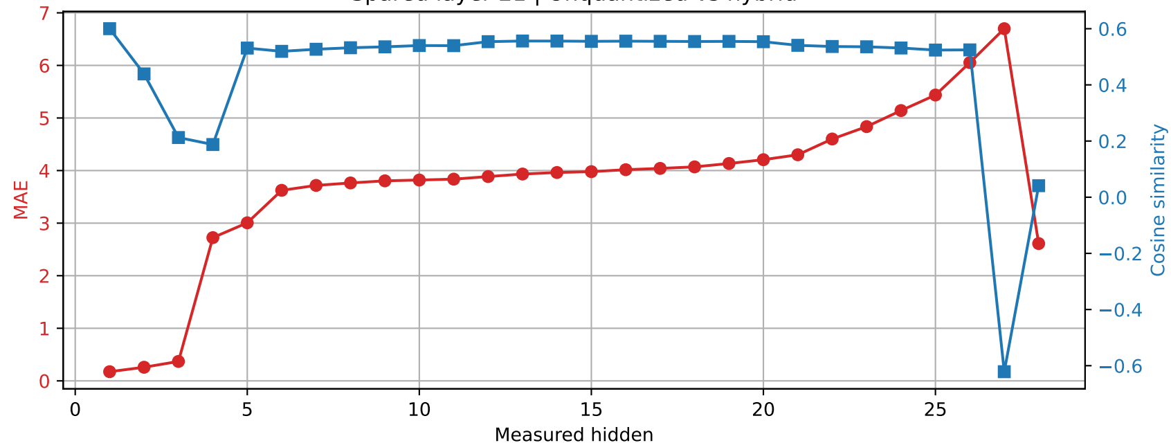
Qwen2.5-7B-Instruct | Prompt 3 Spared layer 21 | Unquantized vs hybrid
