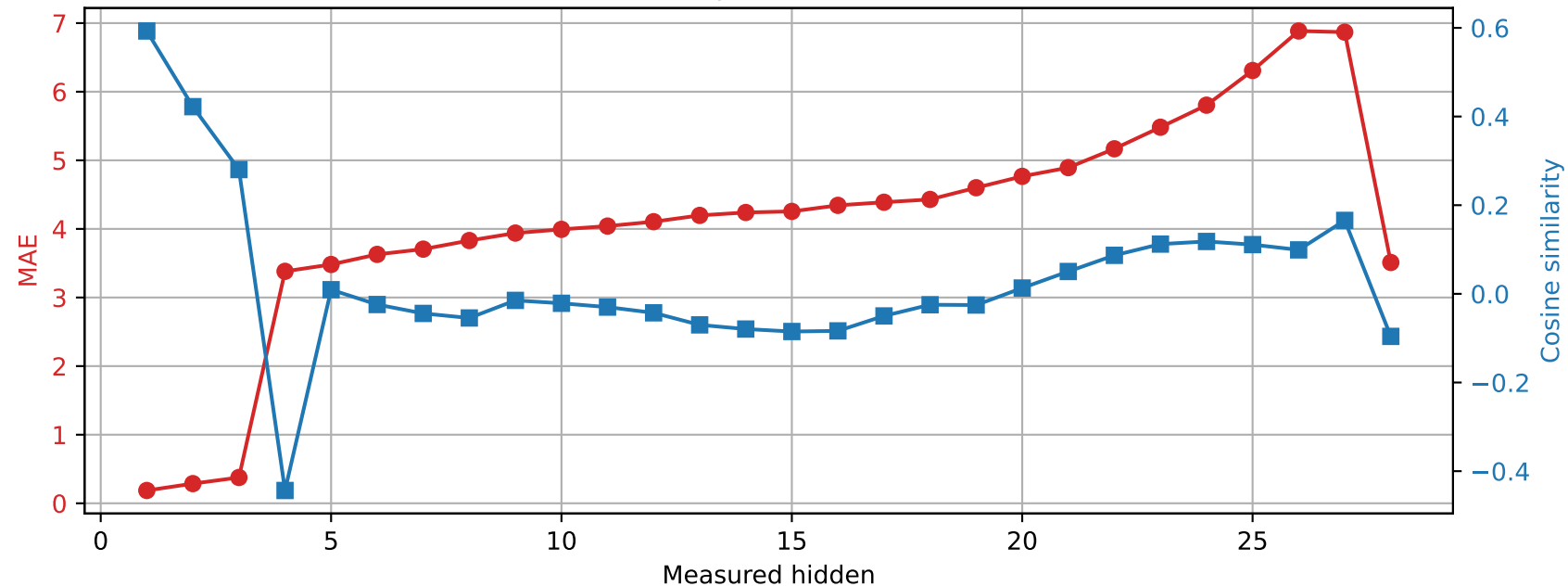
Qwen2.5-7B-Instruct | Prompt 4 Spared layer 24 | Unquantized vs hybrid
