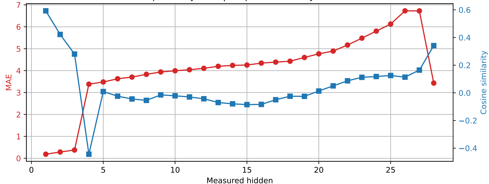
Qwen2.5-7B-Instruct | Prompt 4 Spared layer 27 | Unquantized vs hybrid
