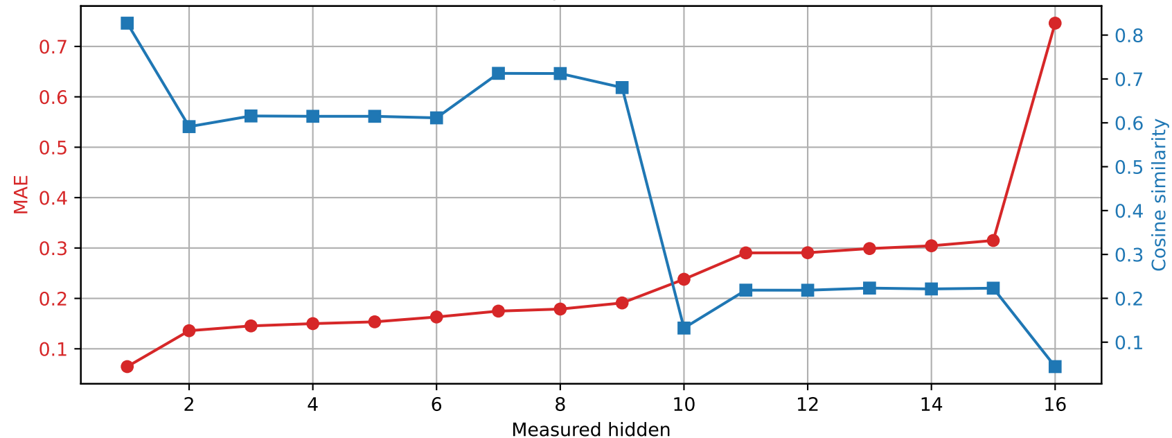
OLMo-1B-hf | Prompt 0 Spared layer 10 | Unquantized vs hybrid
