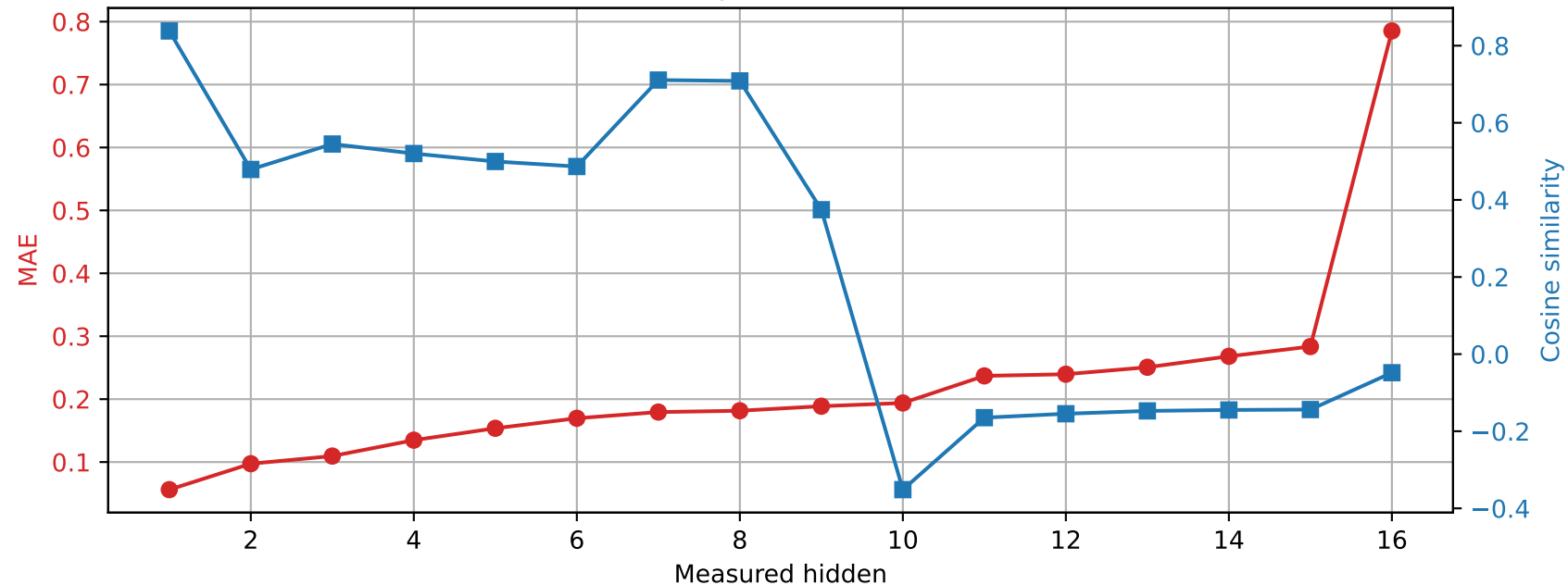
OLMo-1B-hf | Prompt 1 Spared layer 4 | Unquantized vs hybrid
