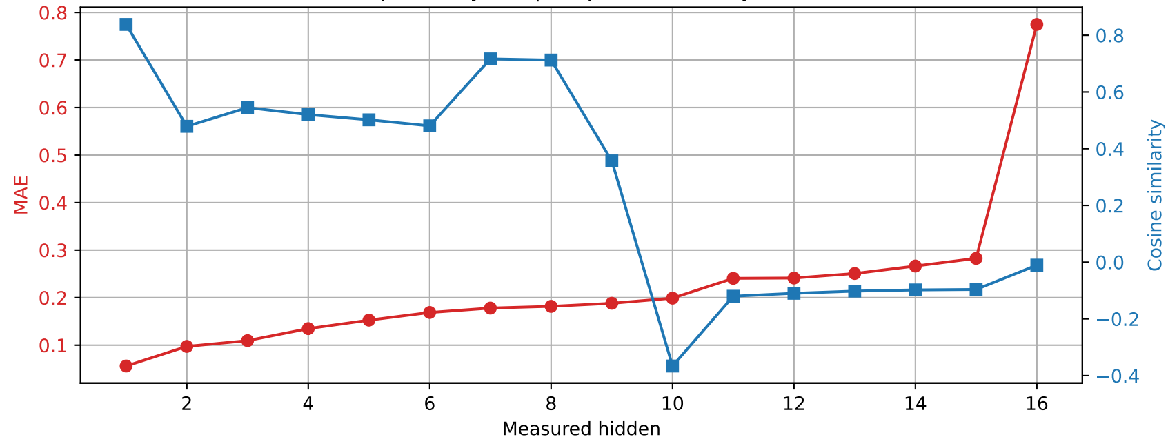
OLMo-1B-hf | Prompt 1 Spared layer 9 | Unquantized vs hybrid
