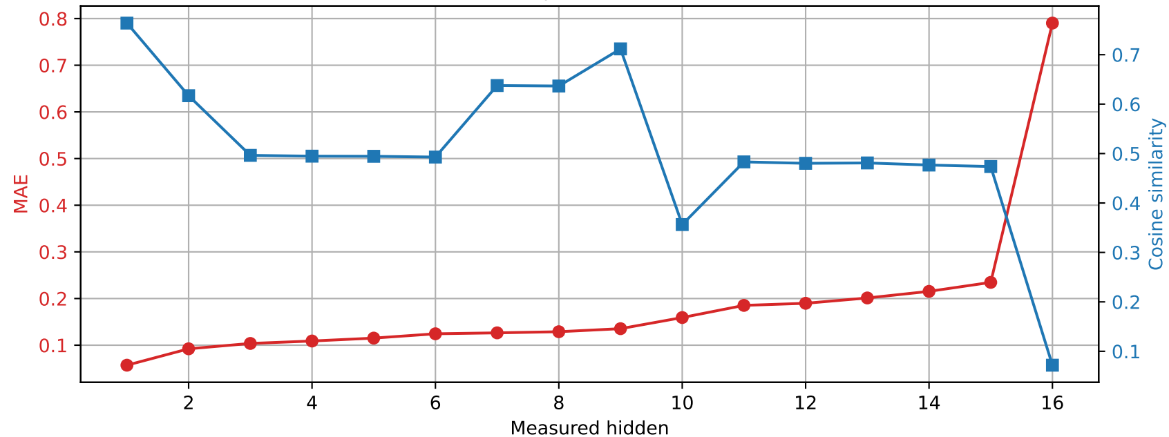
OLMo-1B-hf | Prompt 3 Spared layer 1 | Unquantized vs hybrid
