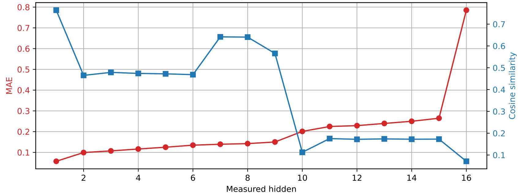
OLMo-1B-hf | Prompt 3 Spared layer 9 | Unquantized vs hybrid
