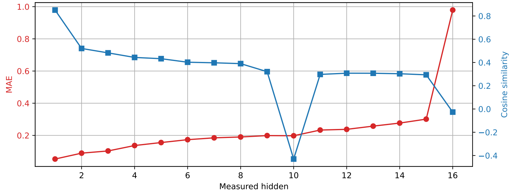
OLMo-1B-hf | Prompt 4 Spared layer 13 | Unquantized vs hybrid
