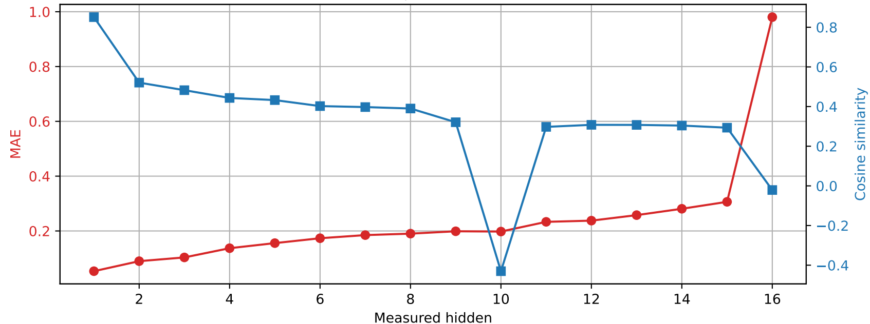
OLMo-1B-hf | Prompt 4 Spared layer 14 | Unquantized vs hybrid
