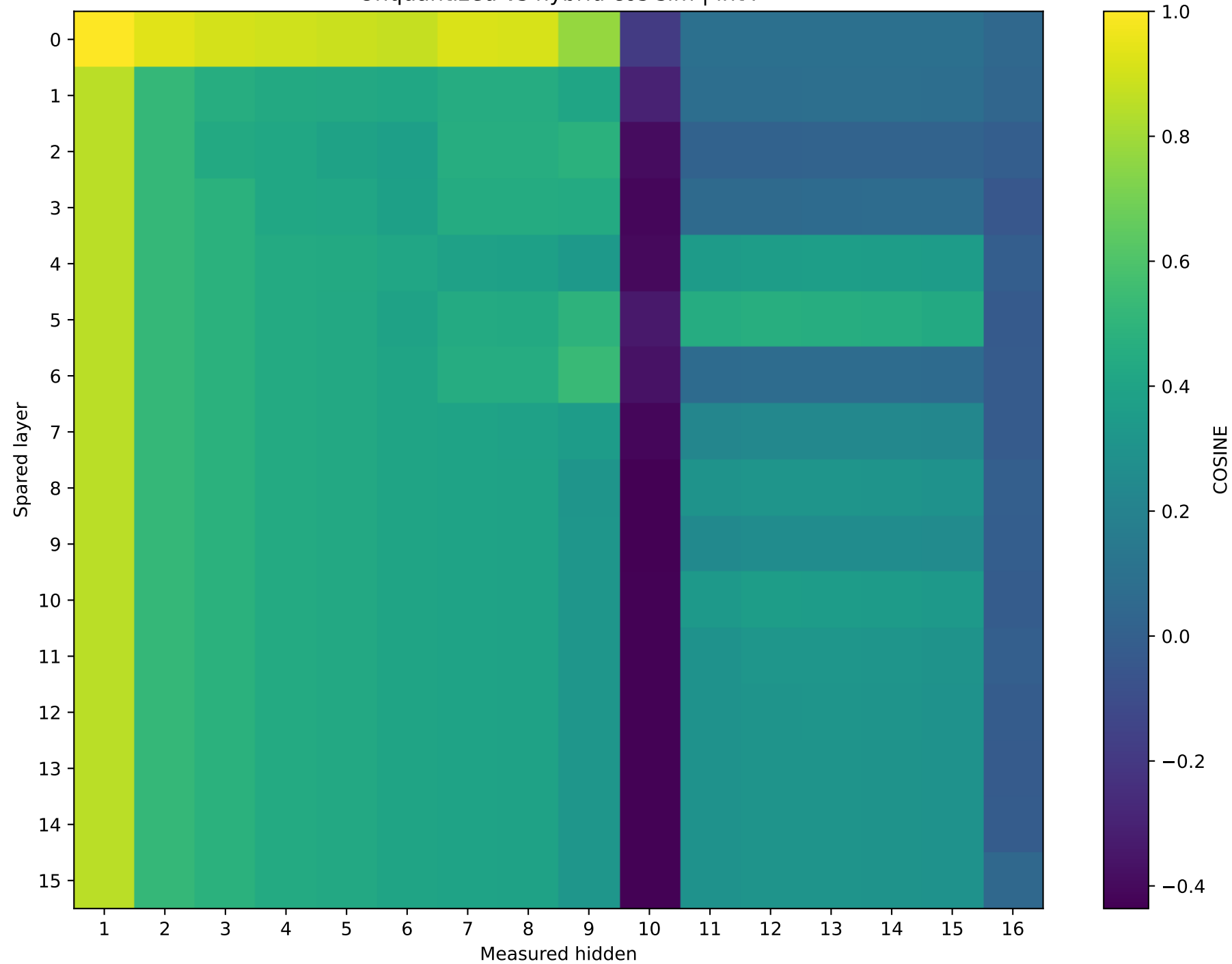
OLMo-1B-hf | Prompt 4 Unquantized vs hybrid cos sim | int4
