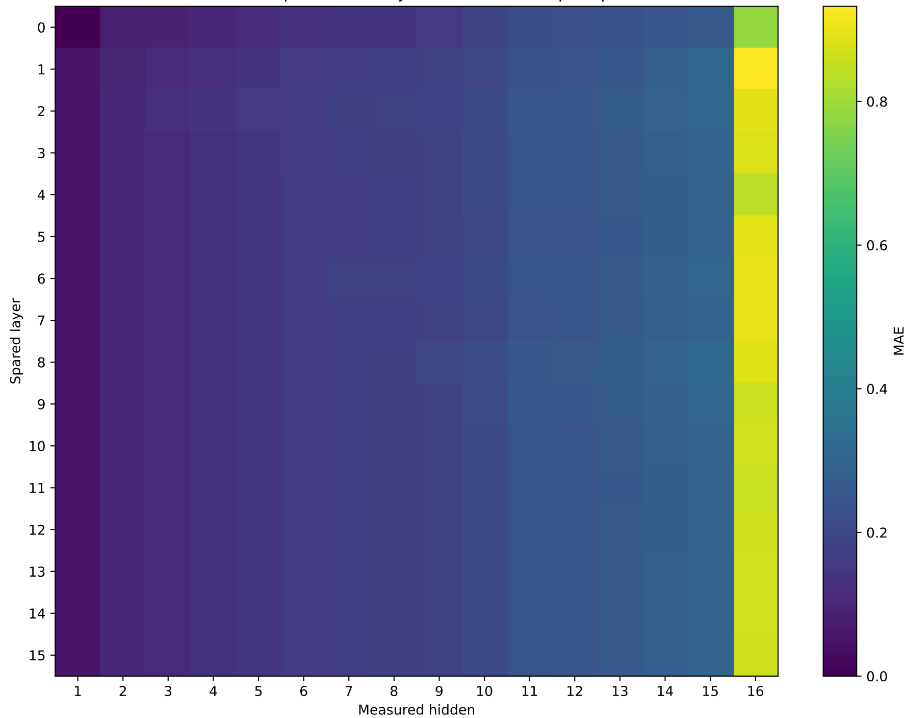
OLMo-1B-hf Mean unquantized vs hybrid MAE across 5 prompts
