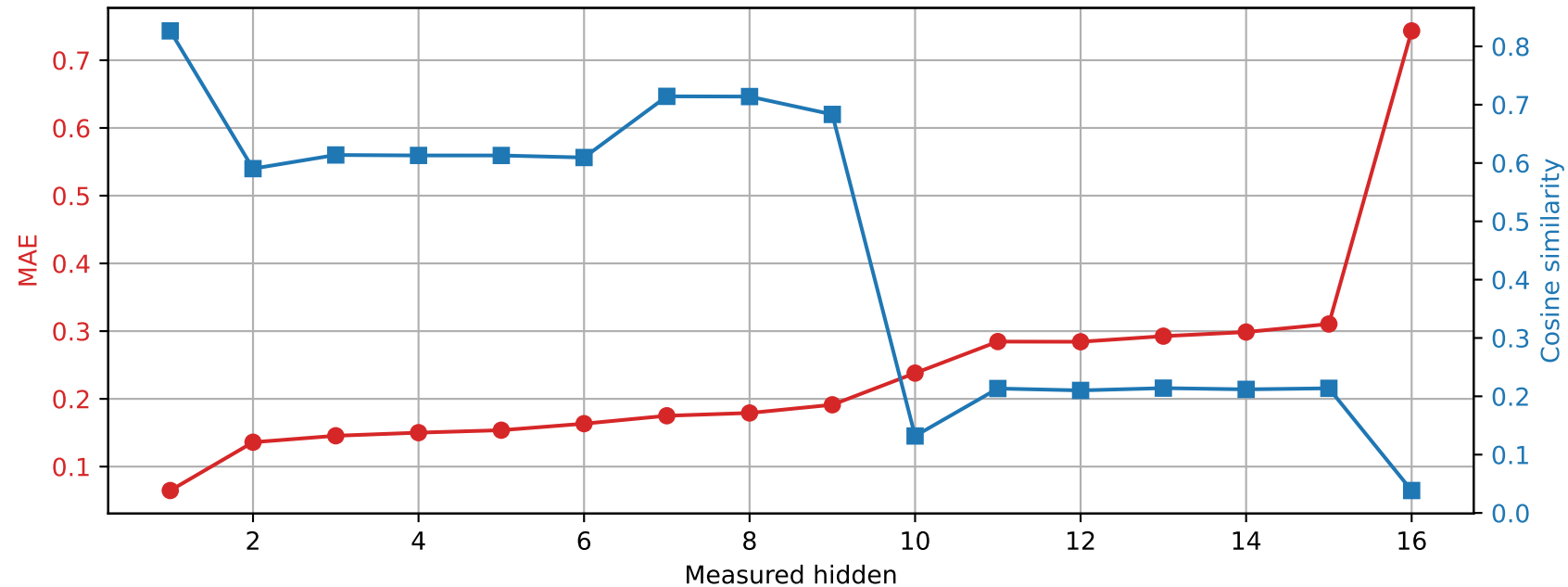
OLMo-1B-hf | Prompt 0 Unquantized vs quantized int4
