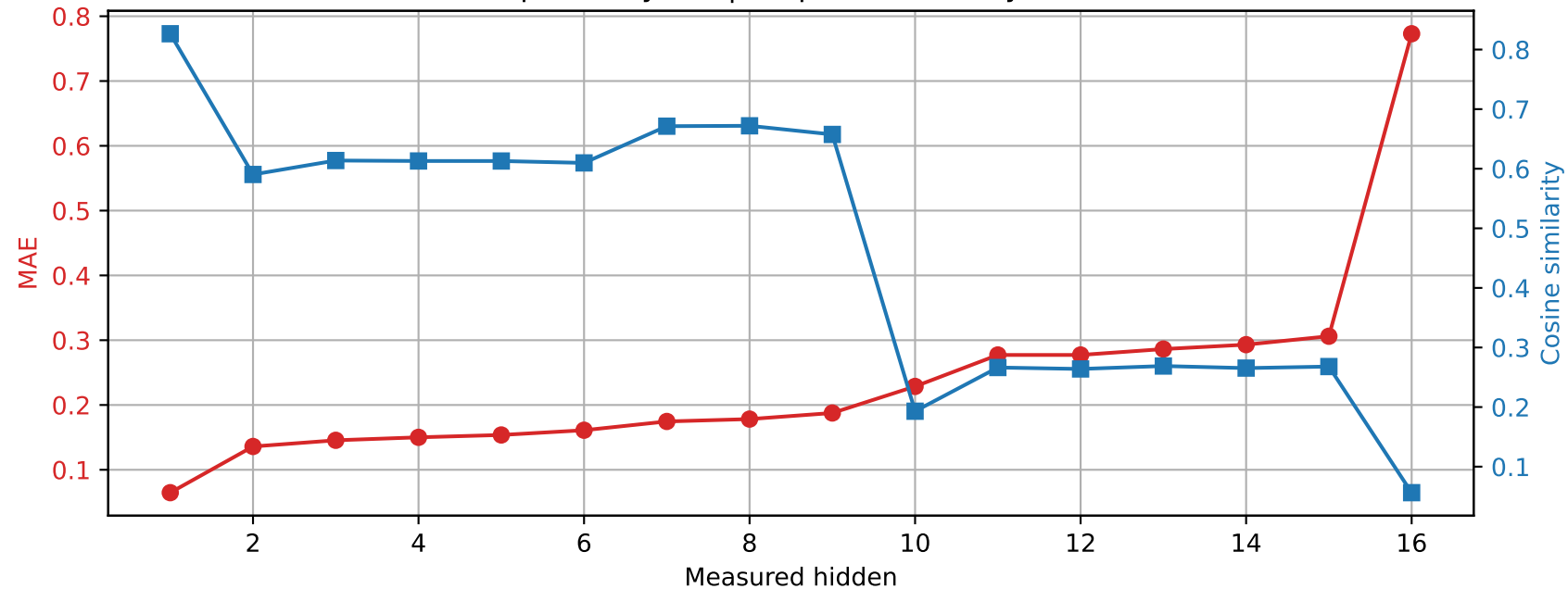
OLMo-1B-hf | Prompt 0 Spared layer 5 | Unquantized vs hybrid
