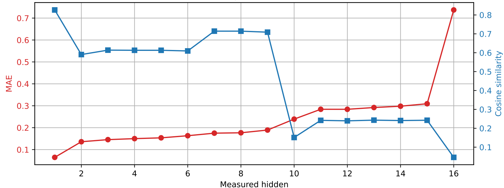
OLMo-1B-hf | Prompt 0 Spared layer 7 | Unquantized vs hybrid
