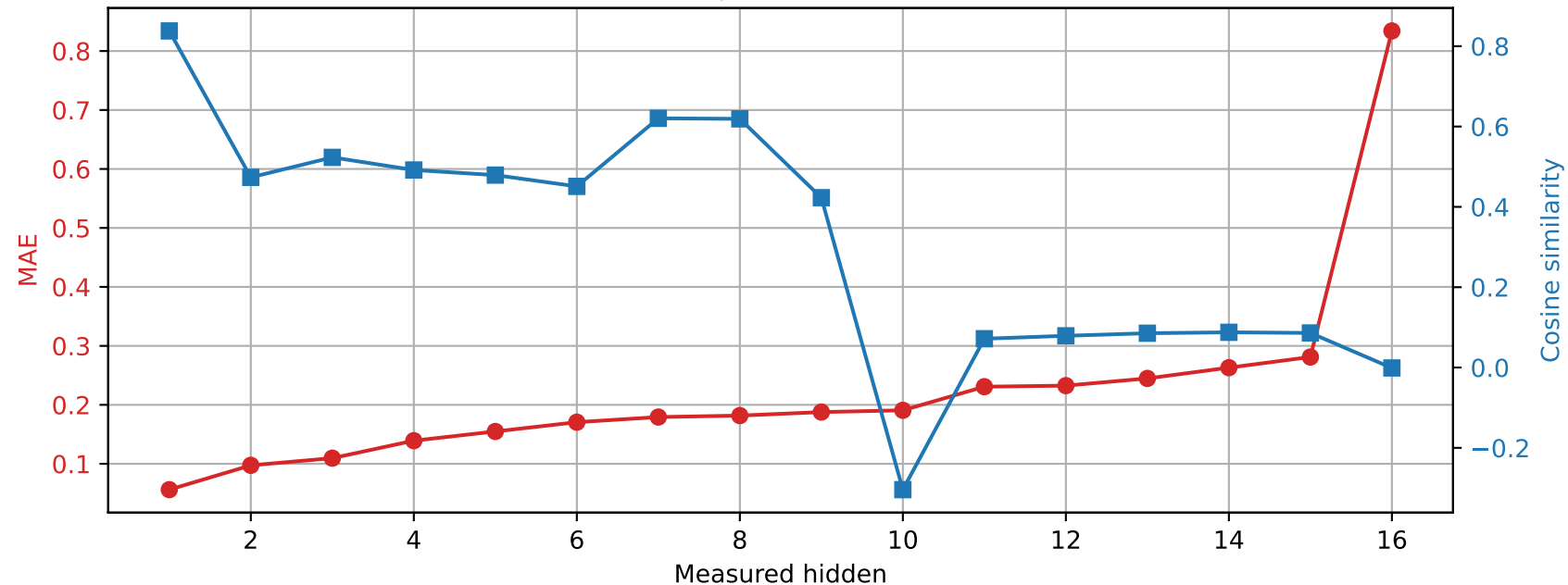
OLMo-1B-hf | Prompt 1 Spared layer 3 | Unquantized vs hybrid
