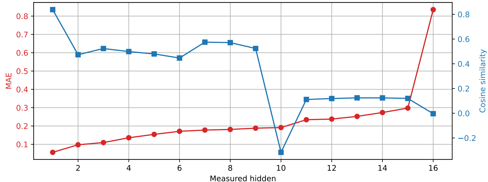
OLMo-1B-hf | Prompt 1 Spared layer 5 | Unquantized vs hybrid
