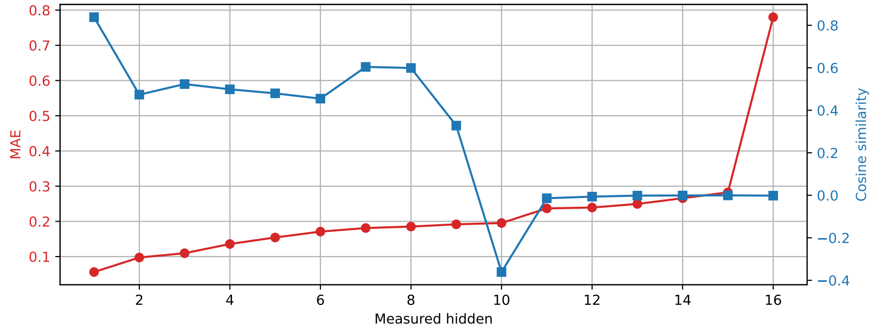
OLMo-1B-hf | Prompt 1 Spared layer 11 | Unquantized vs hybrid
