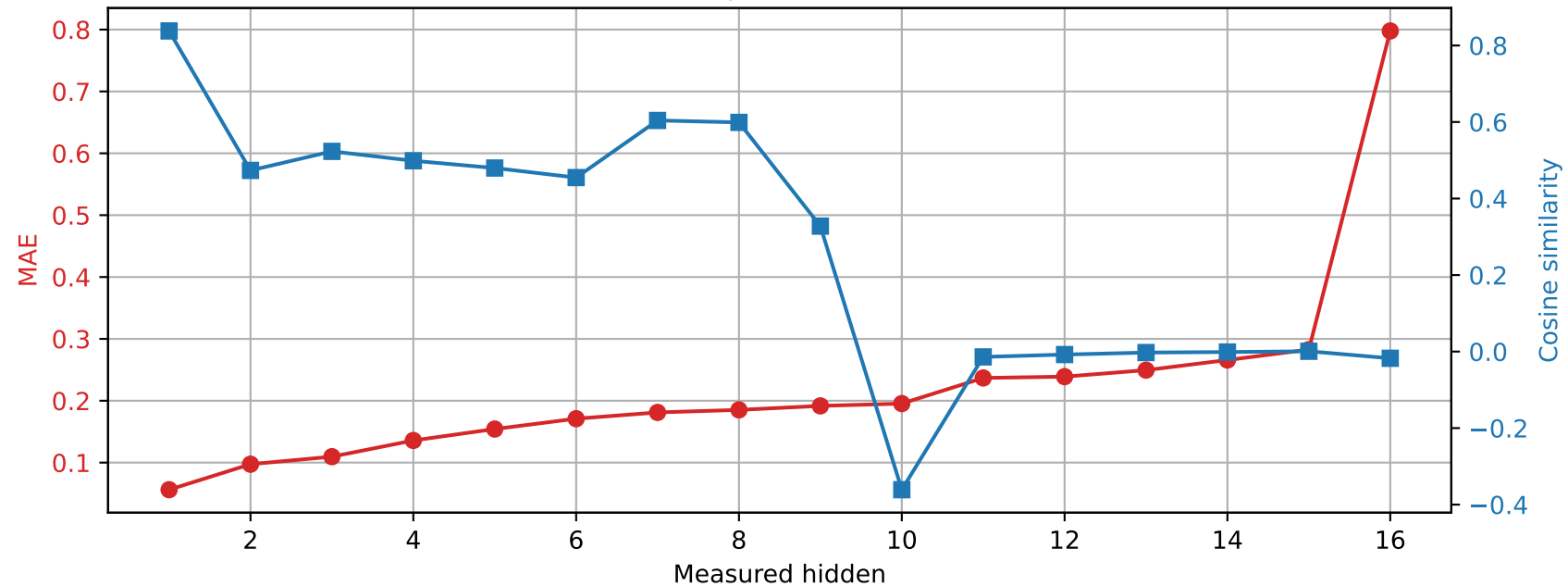
OLMo-1B-hf | Prompt 1 Spared layer 14 | Unquantized vs hybrid
