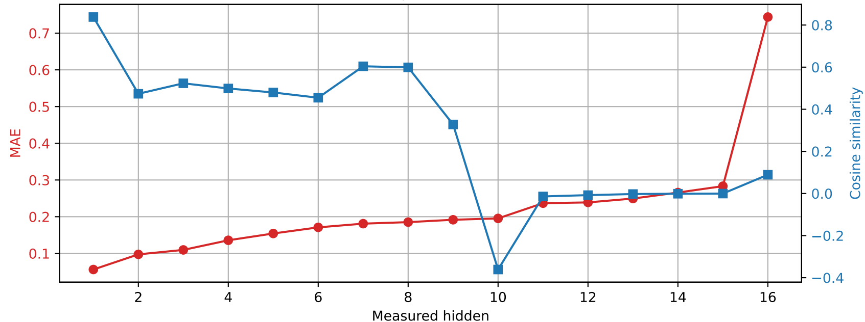
OLMo-1B-hf | Prompt 1 Spared layer 15 | Unquantized vs hybrid
