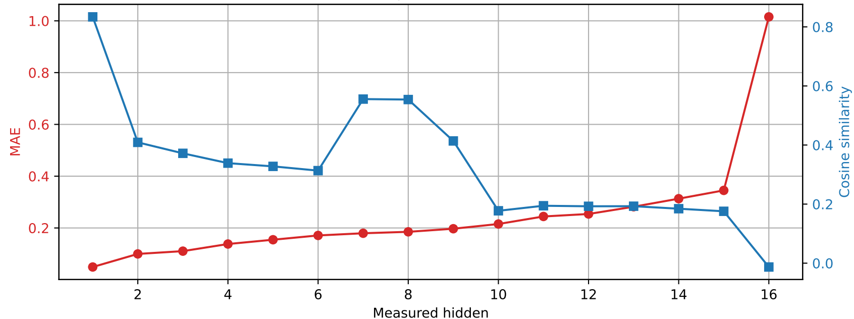
OLMo-1B-hf | Prompt 2 Spared layer 4 | Unquantized vs hybrid
