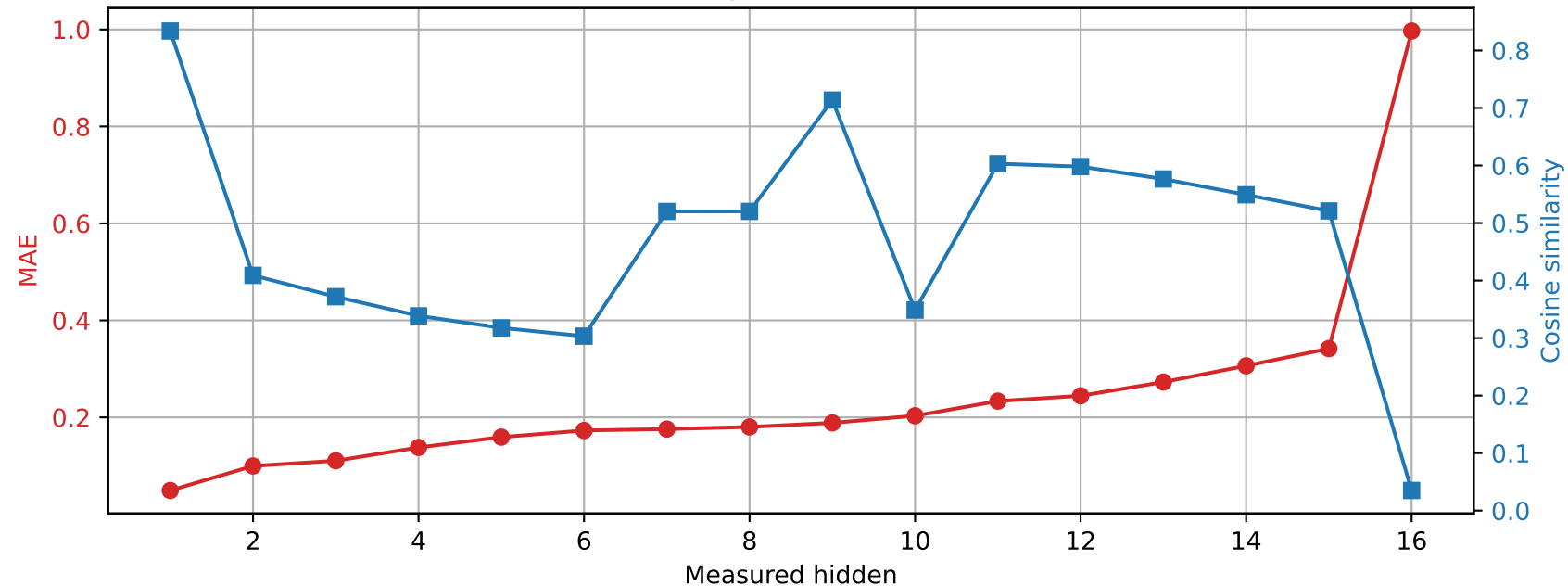
OLMo-1B-hf | Prompt 2 Spared layer 6 | Unquantized vs hybrid
