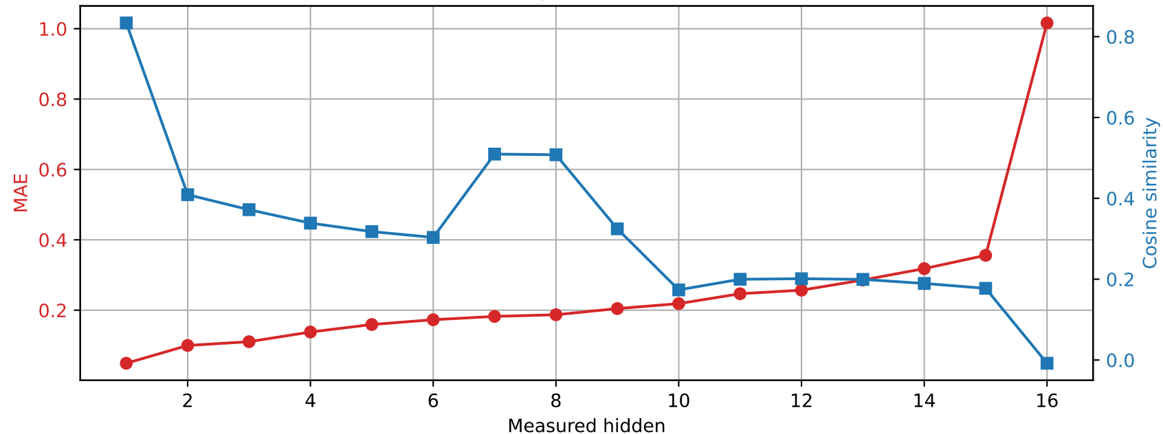
OLMo-1B-hf | Prompt 2 Spared layer 8 | Unquantized vs hybrid
