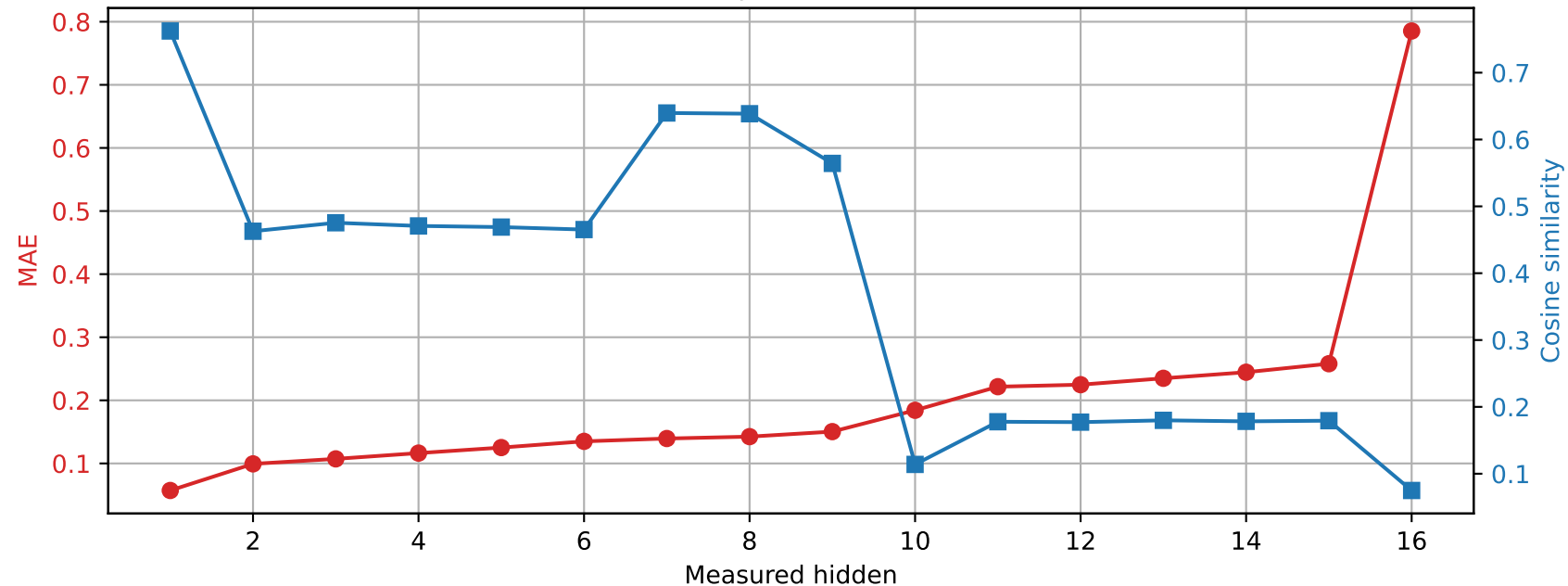
OLMo-1B-hf | Prompt 3 Spared layer 10 | Unquantized vs hybrid
