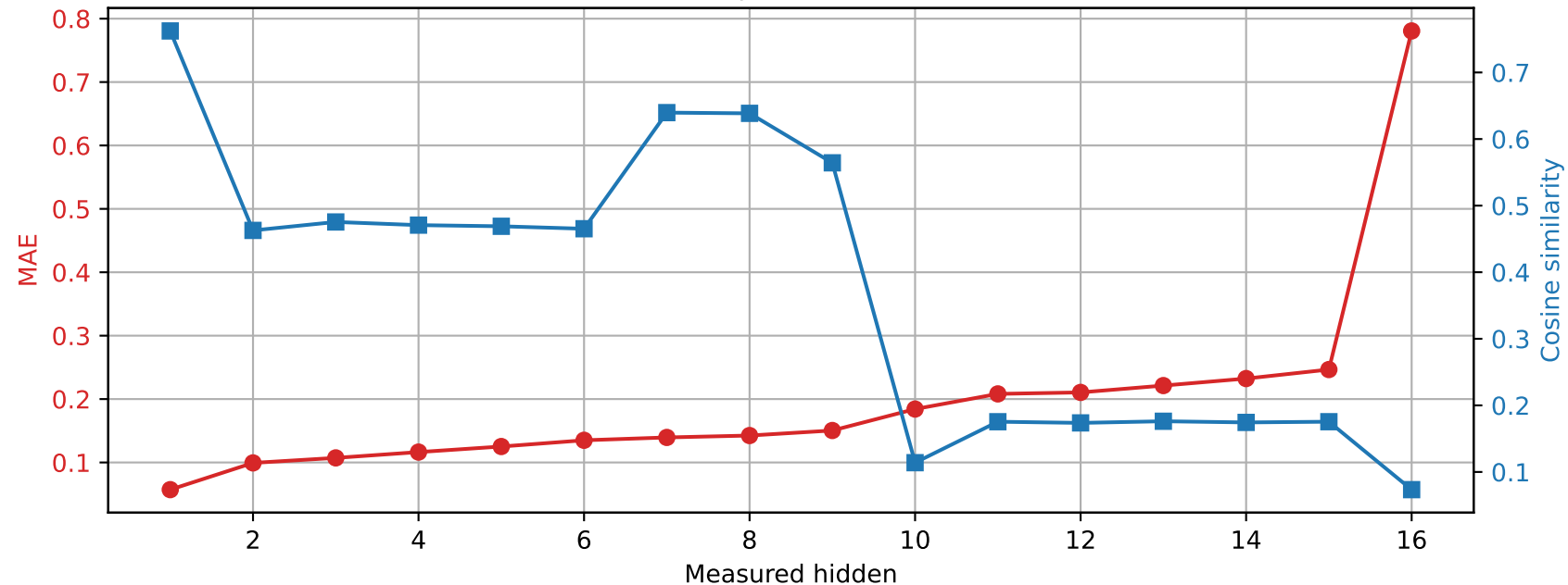
OLMo-1B-hf | Prompt 3 Spared layer 11 | Unquantized vs hybrid
