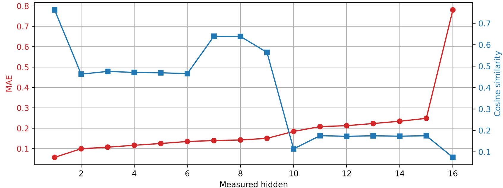
OLMo-1B-hf | Prompt 3 Spared layer 14 | Unquantized vs hybrid
