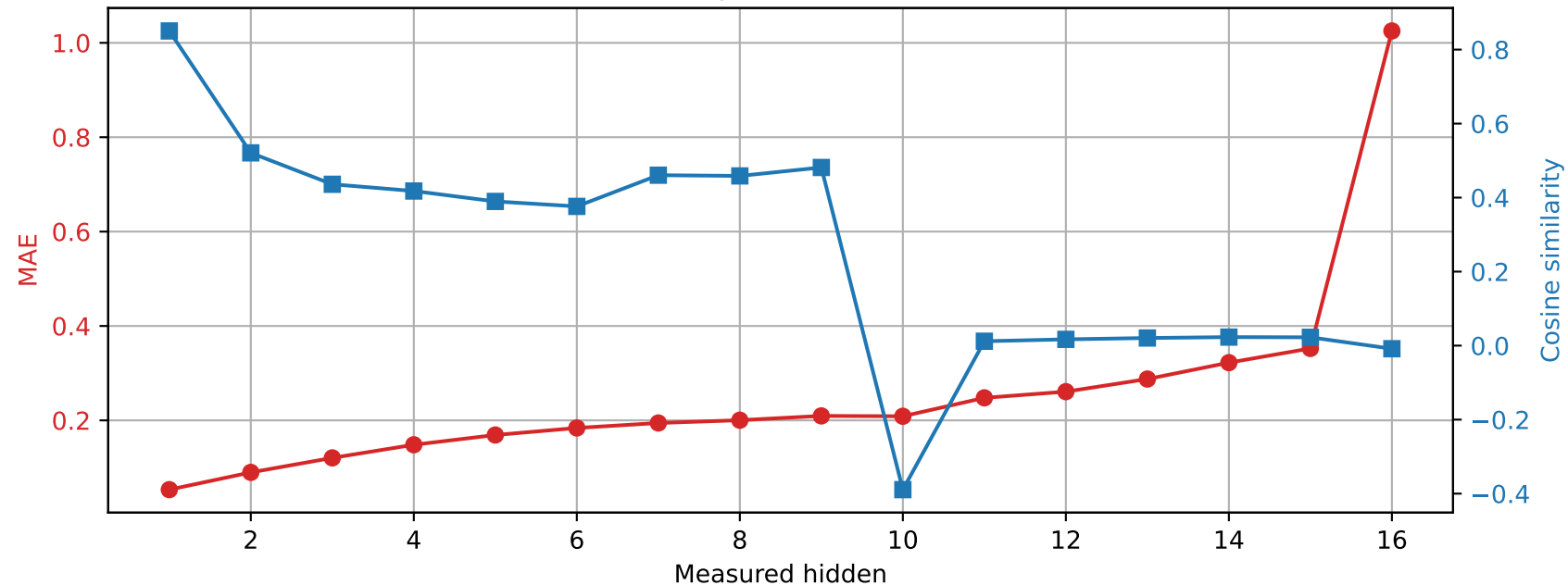
OLMo-1B-hf | Prompt 4 Spared layer 2 | Unquantized vs hybrid
