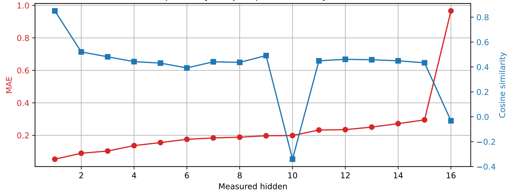
OLMo-1B-hf | Prompt 4 Spared layer 5 | Unquantized vs hybrid
