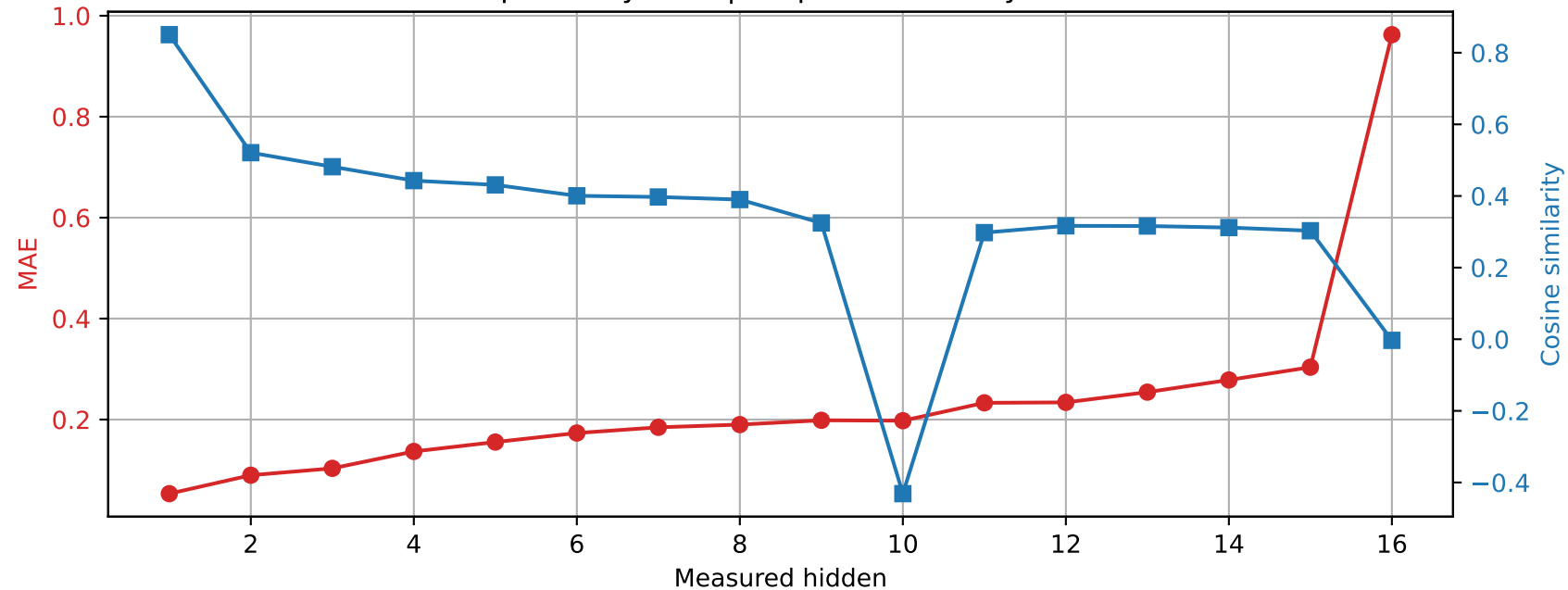
OLMo-1B-hf | Prompt 4 Spared layer 11 | Unquantized vs hybrid
