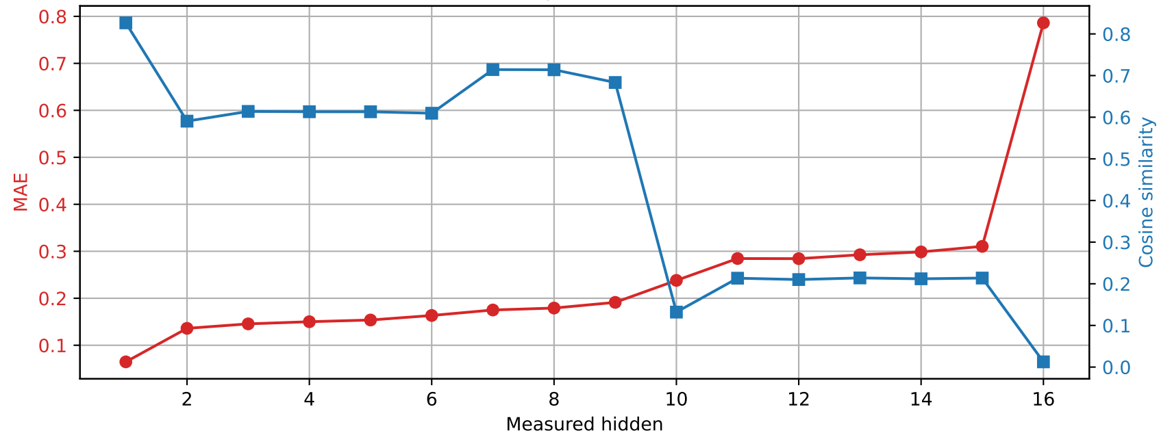
OLMo-1B-hf | Prompt 0 Spared layer 15 | Unquantized vs hybrid
