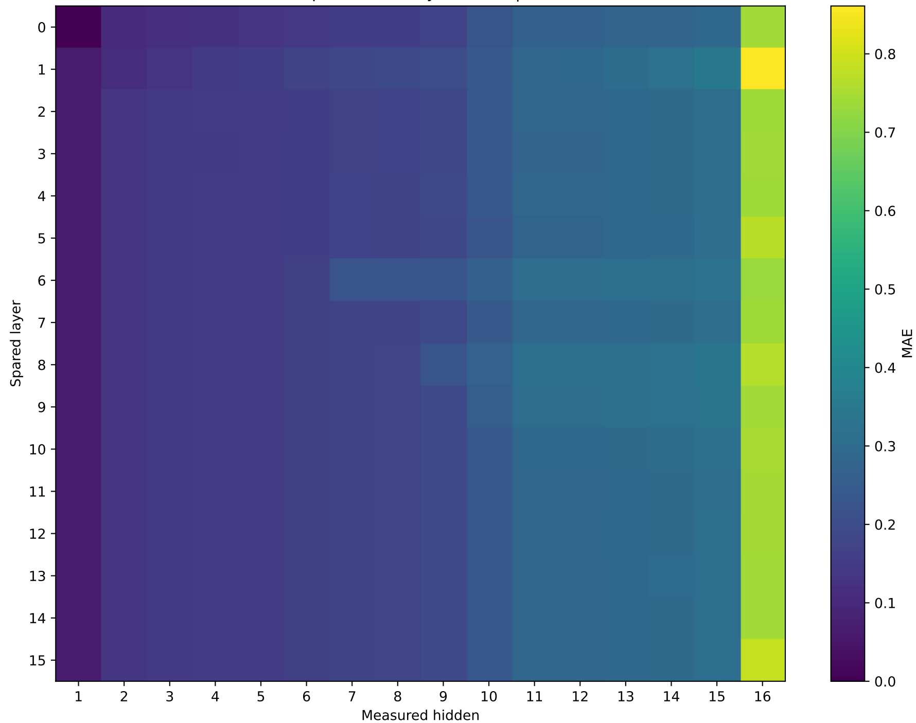
OLMo-1B-hf | Prompt 0 Unquantized vs hybrid MAE | int4
