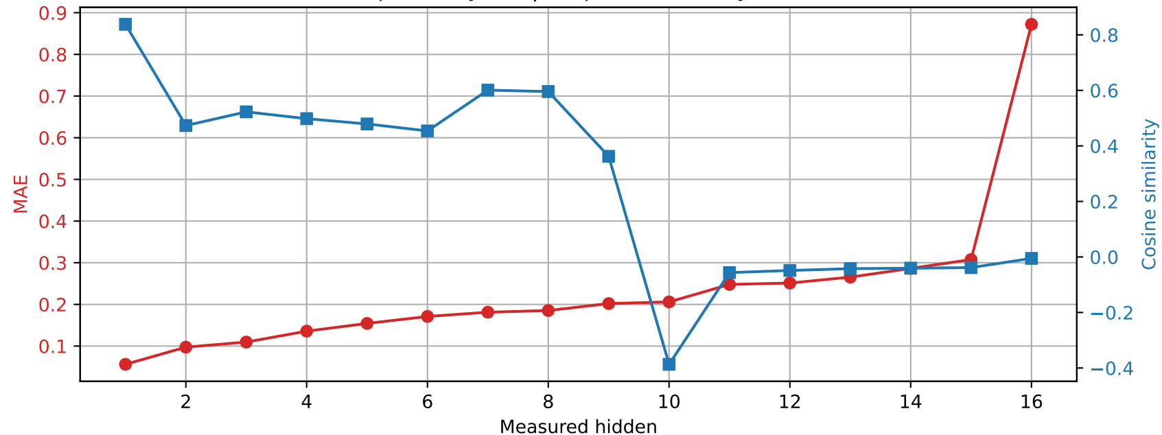
OLMo-1B-hf | Prompt 1 Spared layer 8 | Unquantized vs hybrid
